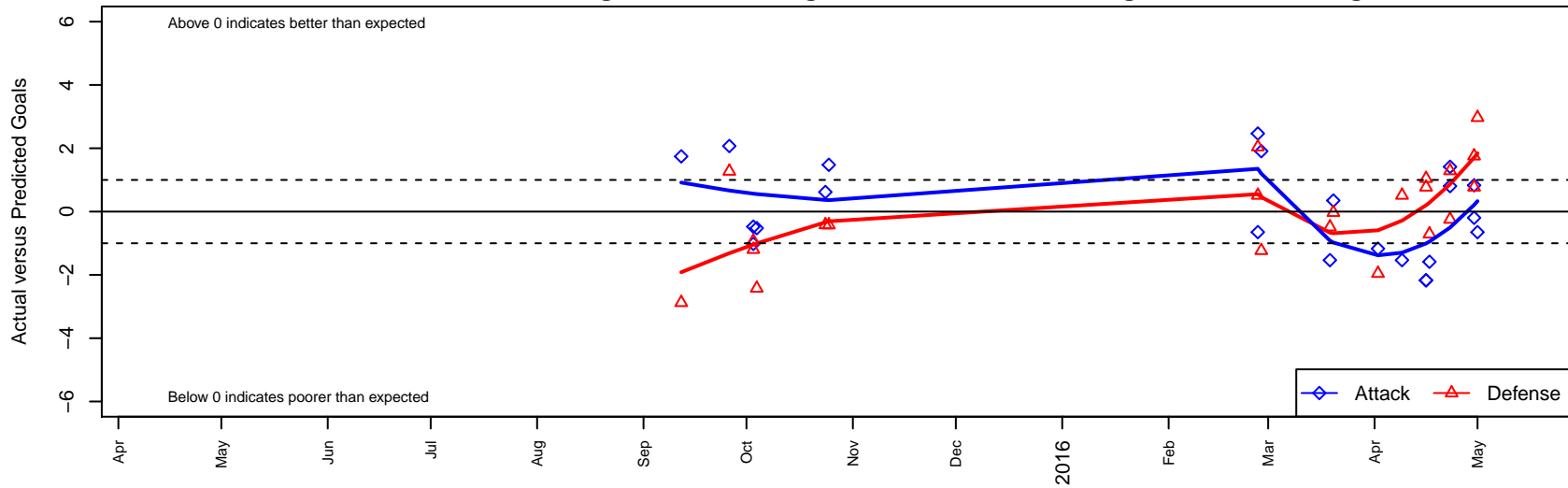
Three Rivers SC Black District G04 Dots are actual minus expected GF (blue circles) and GA (red triangles). Blue line is smoothed change in attack strength. Red is smoothed change in defense strength.
